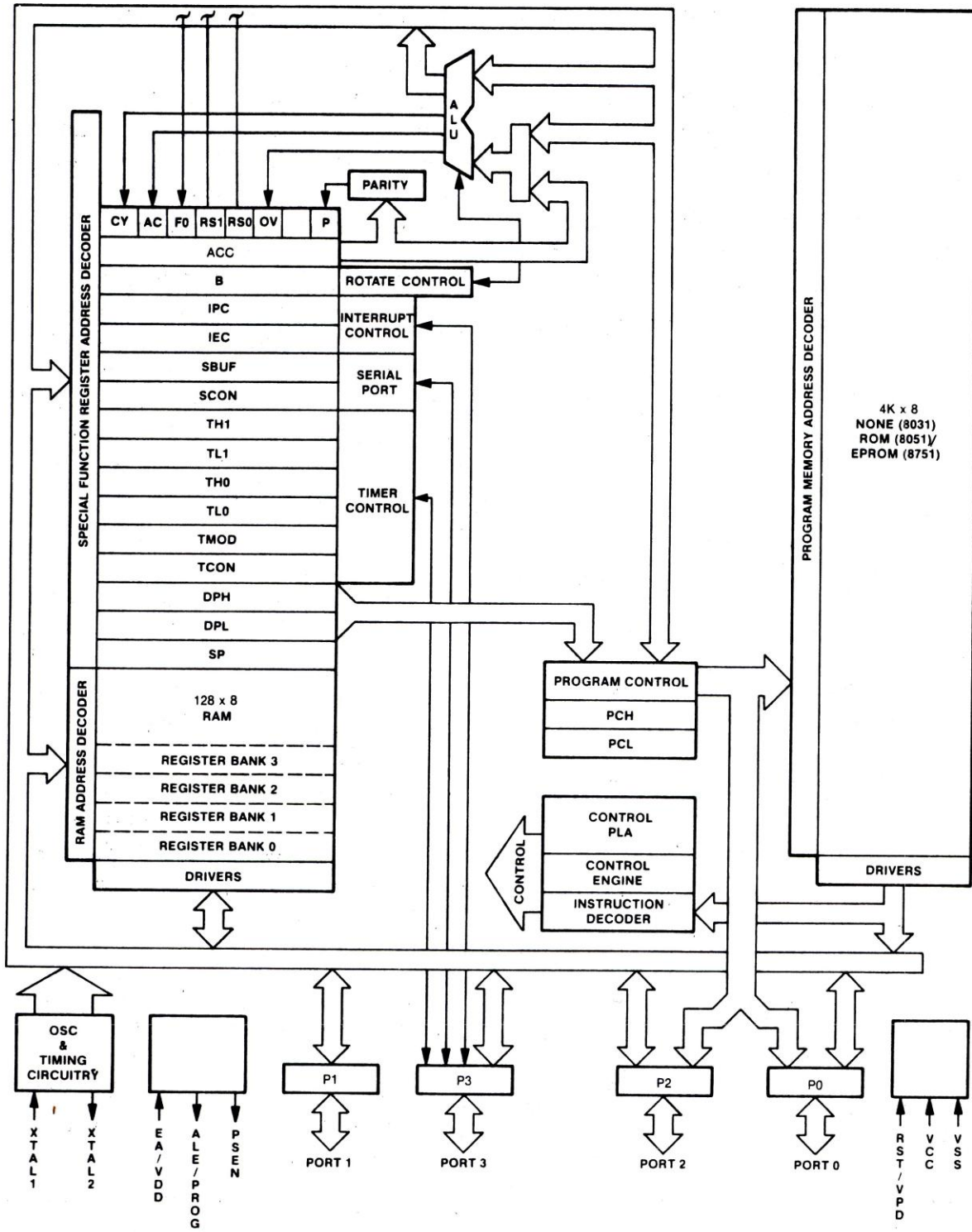
8051 Architecture |
